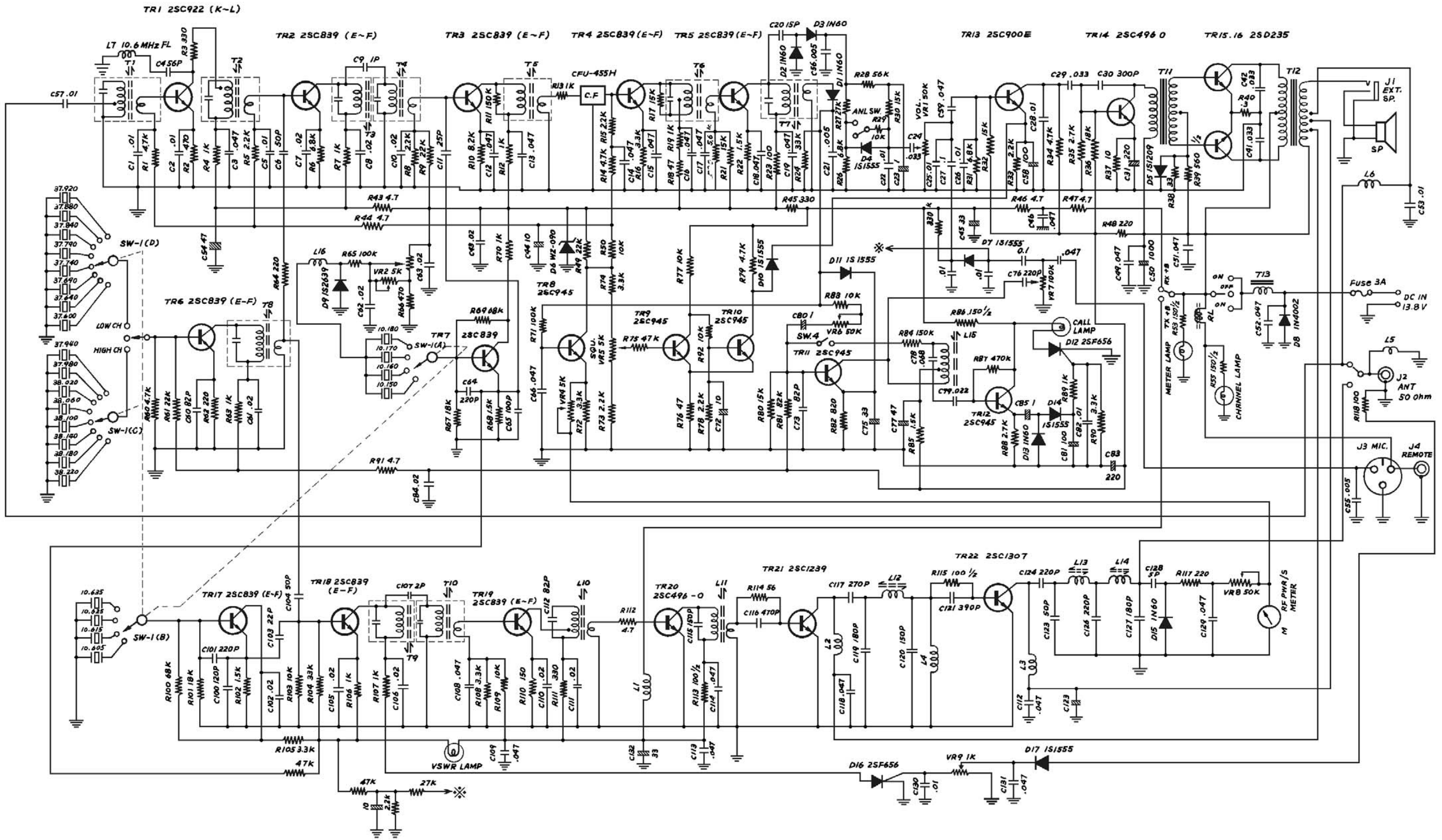
Sommerkamp Model TS-660S
